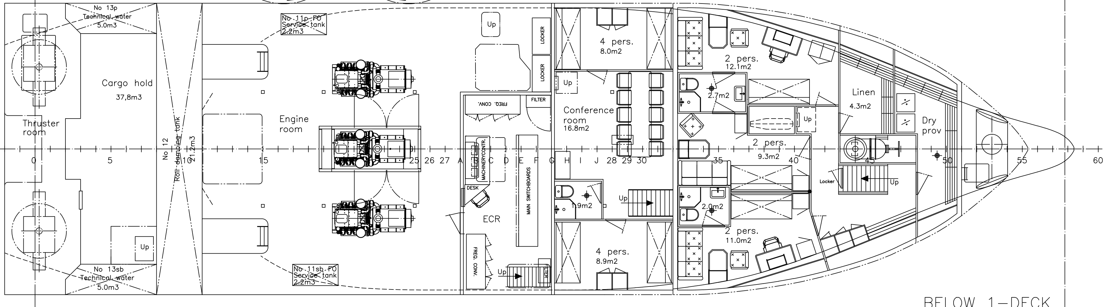
BELOW 1-DECK
